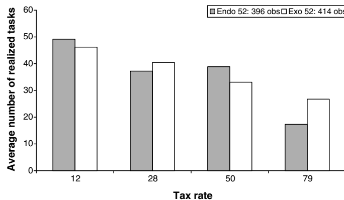
Fig. 5b. Average work by tax rate (range [0–52]).
