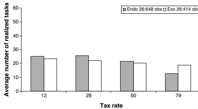
Fig. 5a. Average work by tax rate (range [0–26]).
