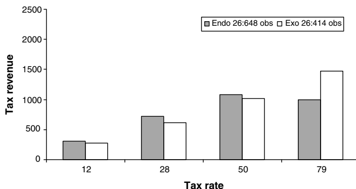
Fig. 1a. Variation of tax revenue by tax rates (26 tasks).
