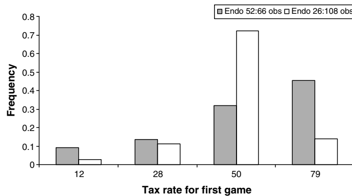
Fig. 4. Frequency of choice of tax rates by tax setters in the first game in endogenous treatments.
