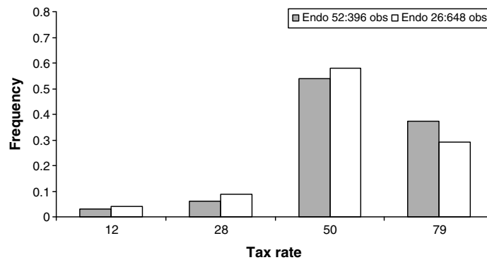
Fig. 3. Frequency of choice of tax rates by tax setters in the endogenous treatments.
