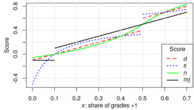
FIGURE 3 Score of each rule given the following distribution of grades : 10% of -1 , 10% of +2 , the abscissa x of +1 , and the remaining of 0.
