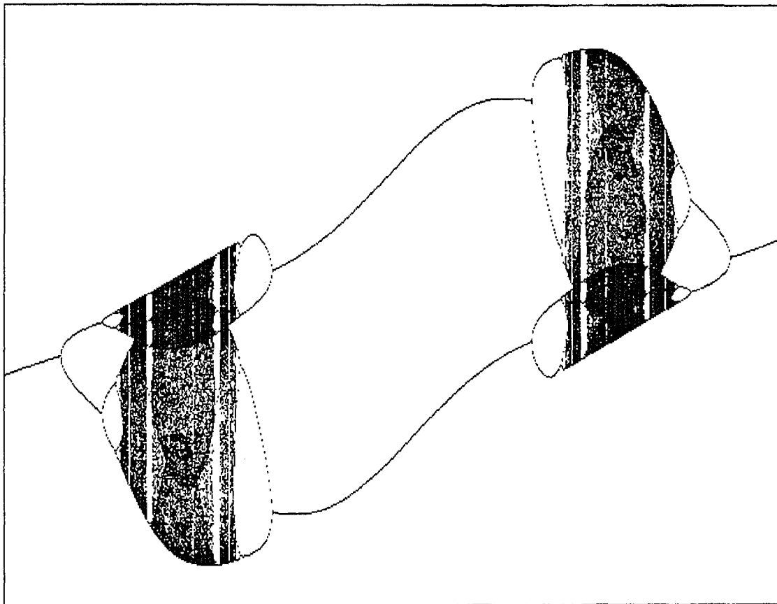
Fig. 1. Shifting the demand curve upwards, stable periodic and chaotic price behaviour may interchange several times.
