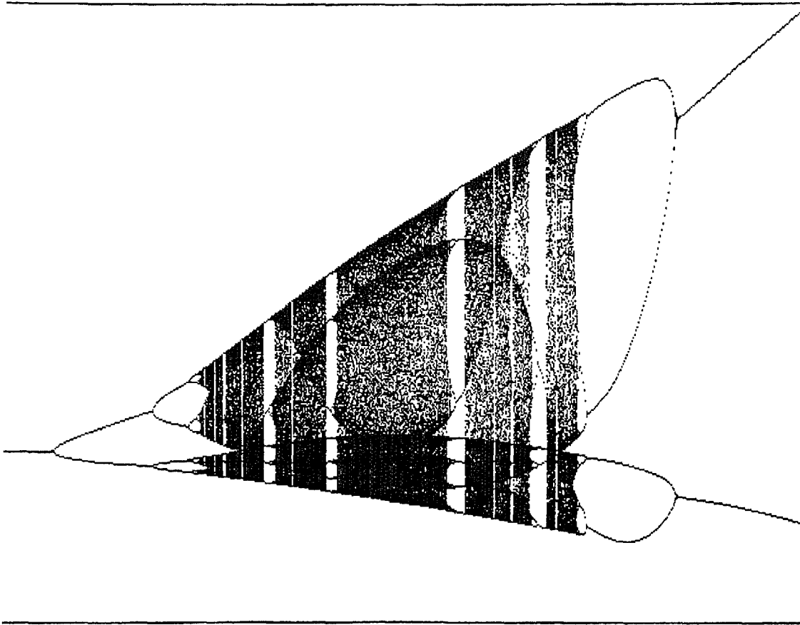
Fig. 2. For w close to 0 a stable equilibrium occurs, while for w close to 1 stable period 2 oscillations with large amplitude arise; for intermediate values of w chaotic price oscillations with moderate amplitude arise.
